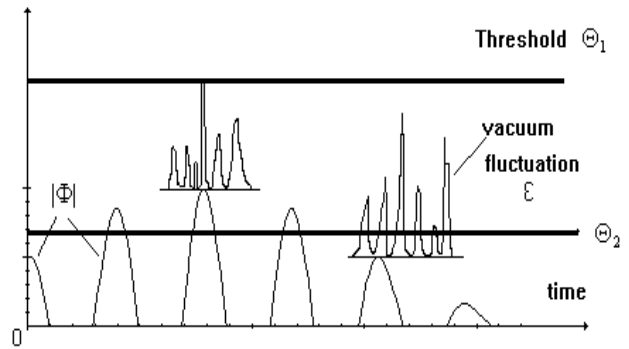
Fig. 4. Quantum measurements.
