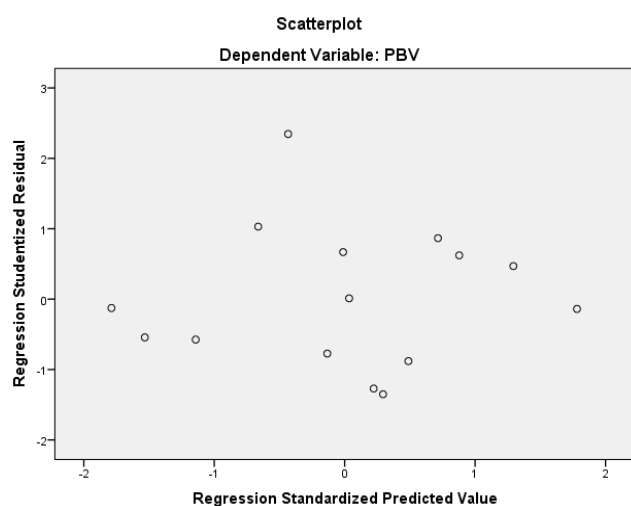
Figure 1. Heteroscedasticity Test.
