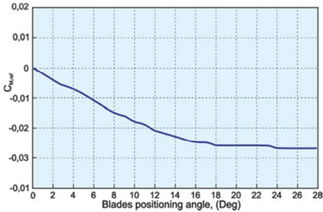
Figure 6. Moment coefficient C_{M,ref} depending on the angle of attack for the NACA 0016 profile.
