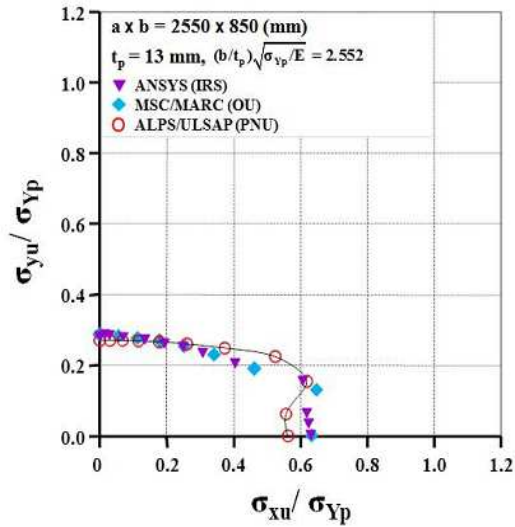
(a) Plate with t_p = 13 \text{ mm}
