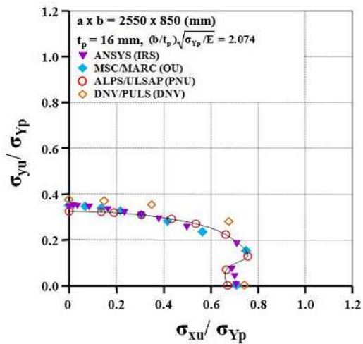
(b) Plate with t_p = 16 \text{ mm}
