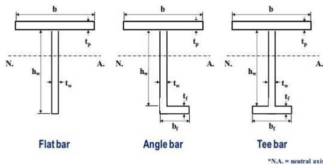
Figure 6. Nomenclature of Stiffened panel
