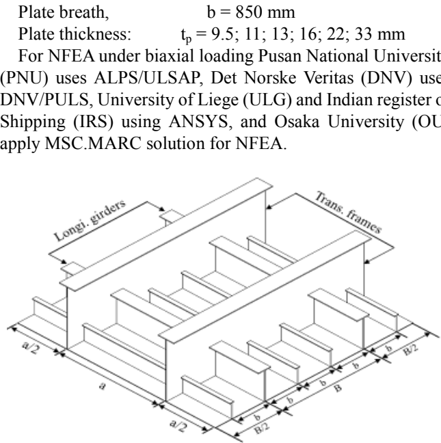
Figure 5. Stiffened panel in NFEA
