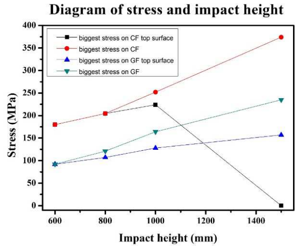
Figure 7. Connection of stress and impact height.
