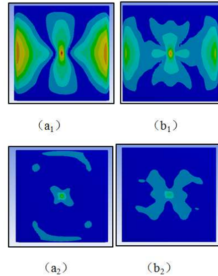
Figure 4. h=800\text{mm} .
