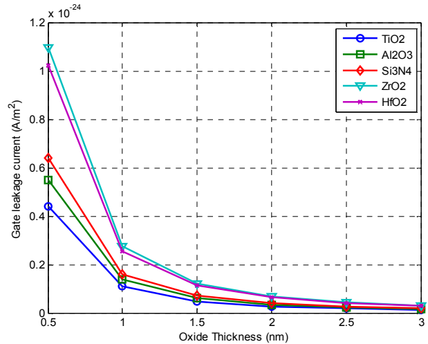
Figure 4. Gate leakage current of different insulating materials.
