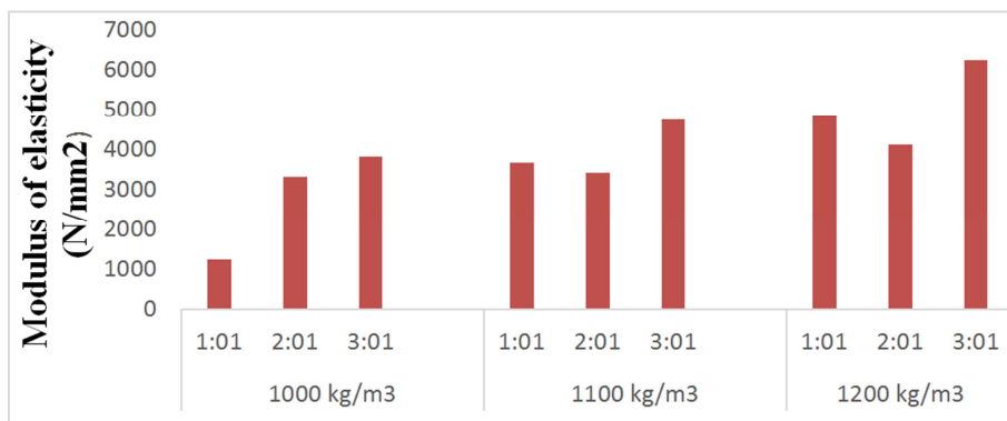
Figure 3. Effect of density and mixing ratio on Modulus of Elasticity of the paper plastic board.
