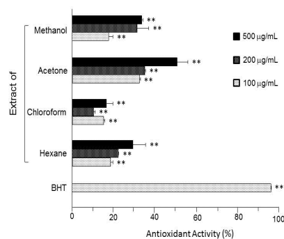
Figure 2. The results of the MA/GC assay on samples prepared by Soxhlet extraction. Values are means \pm SD (n = 3). *: p < 0.05 , **: p < 0.01 .
