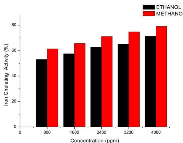
Figure 3. Iron ( Fe^{2+} ) chelating activity of ethanolic and methanolic extracts of peanut hulls. Results are average of triplicate determinations \pm Standard deviation
