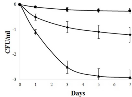
Figure 5. Kinetic of inactivation of E. coli O157:H7 by L. delbrueckii in NB submerged cocultivation and in at 5°C.
