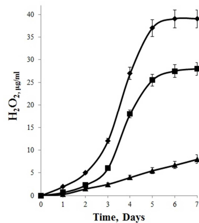
Figure 3. Kinetic of hydrogen peroxide production by L. delbrueckii MDC 9617 at 5°C in beef broth. Cell concentration CFU/ml (◆) 2 \times 10^8 , (■) 6 \times 10^7 , (▲) 3 \times 10^7 .
