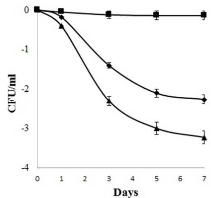
Figure 6. Kinetic of E. coli O157:H7 inactivation by L. delbrueckii MH 10 in ground meat at 5°C. (■) – E. coli O157:H7, (♦) E. coli O157:H7 + 10^7 L. delbrueckii MH 10, (▲) – E. coli O157:H7 + 10^8 L. delbrueckii MH 10.
