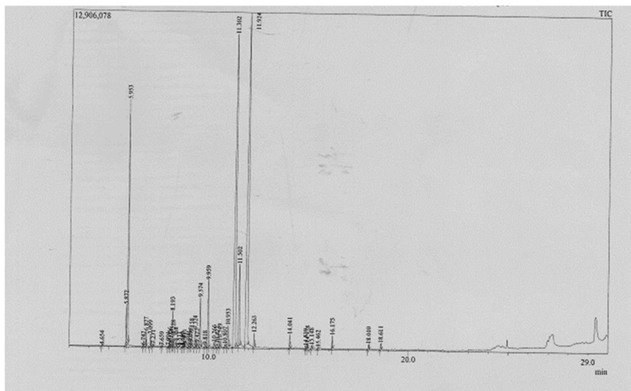
Figure 2. Chromatogram of lemongrass oil obtained from GC/MS.
