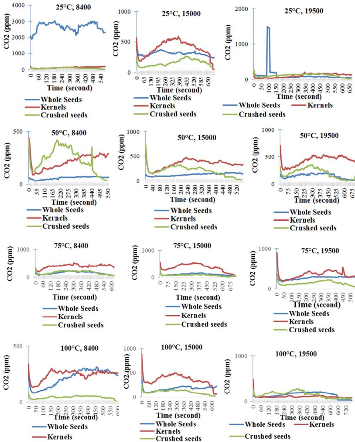
Figure 5. Carbon dioxide as a function of time.
