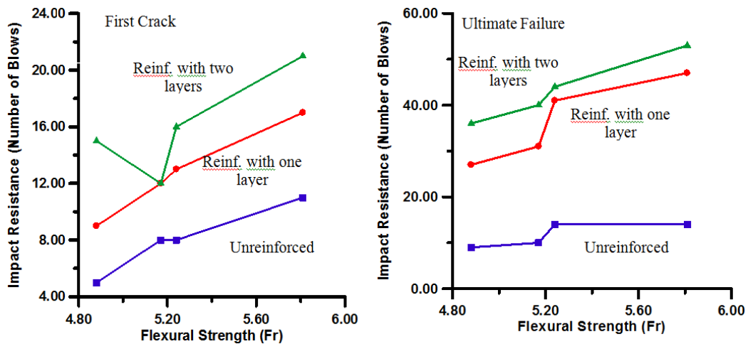
Fig. 14. Relationship Between Flexural Strength and Impact Resistance for First Crack and Ultimate Failure for Ferrocement Specimens at (56) Days for 1.2 m High Falling Mass.
