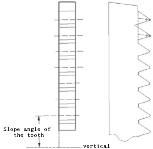
Figure 13. The geometric meaning of slope angle of the tooth.
