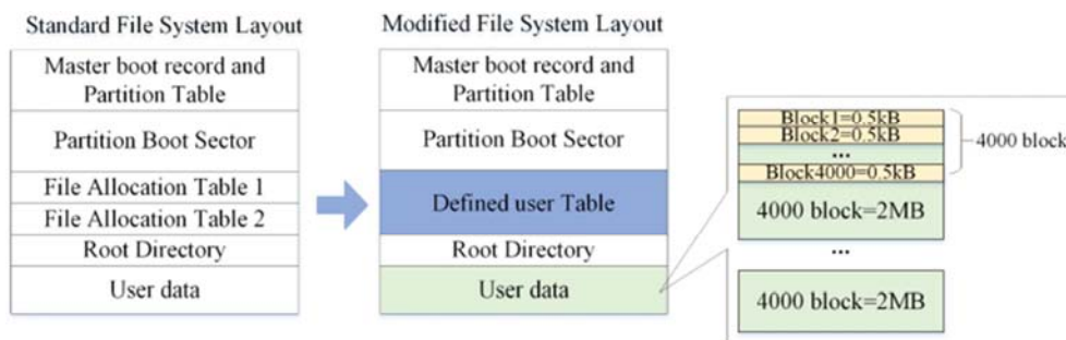
Figure 6. The modified file system.
