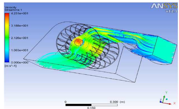
Figure 7. Velocity stream flow with various views.
