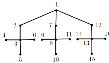
Figure 6. (3,5) -banana tree.
