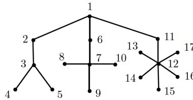
Figure 5. (4,5,7) -banana tree.
