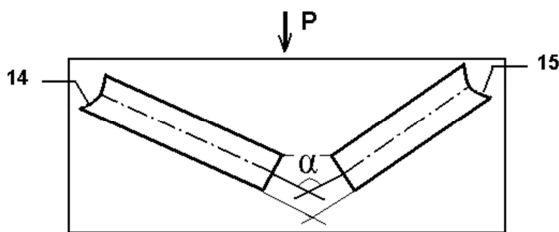
Figure 2. Light conductor 14,15; a_L -poteri in the measuring channel dB. shows the curve of Conditionally fibers under the influence of the load P on a solid structure.
