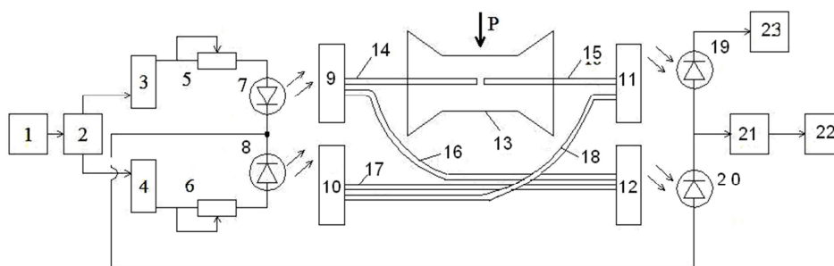
Figure 1. The master oscillator 1; Trigger - ; power amplifiers - 3,4; tokoreguliruyuschie registry - 5,6; light-emitting diodes 7,8, nesimmitrichnye connectors - 9,10,11,12; solid-state design, 13; Sensor fibers - 14,15,16,17,18; photodetectors - 19,20; photoelectric signal processing unit - 21; computer - 22; Power Supply - 23. The device for the diagnosis of pre-fracture and deformation of solid structures. The device is a two channel - measuring and reference.
