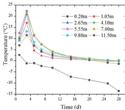
Figure 4. Pile center.
