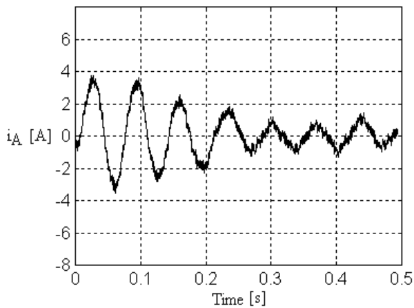
b) R_r=3,2 \Omega (cage made of copper)
