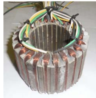
Figure 11. Exterior view of the 24-phase induction motor stator developing according to the drawing shown in Figure 9.
