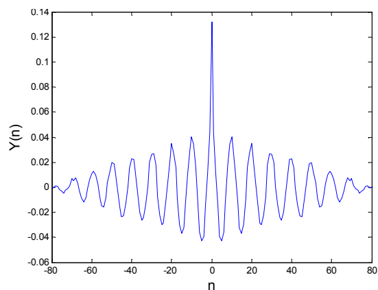
Figure 4. Auto-correlation function of incoherent LFM burst.
