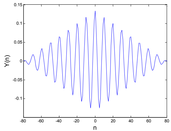
Figure 3. Auto-correlation function of coherent LFM burst.
