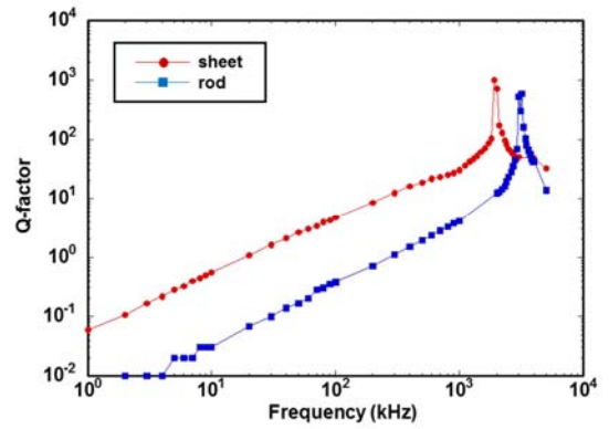
Figure 6. Evaluated Q-factor.
