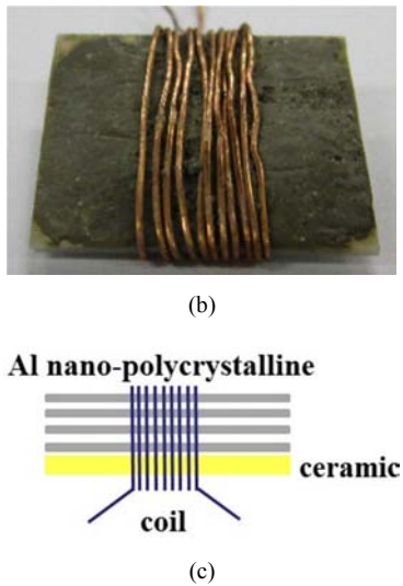
Figure 1. Fabricated cored inductor with Al nano-polycrystalline substance. (a) Low volume resistivity (metal), (b) High volume resistivity, (c) Structure (corresponding to Figure 1a).
