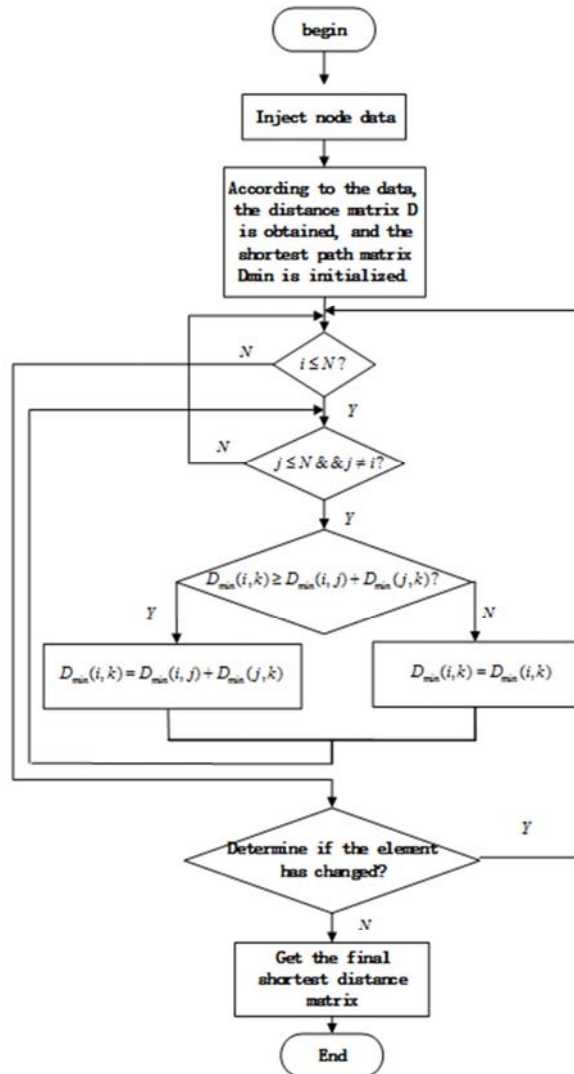
Figure 2. Flow chart for calculating electrical distance based on Floyd algorithm.
