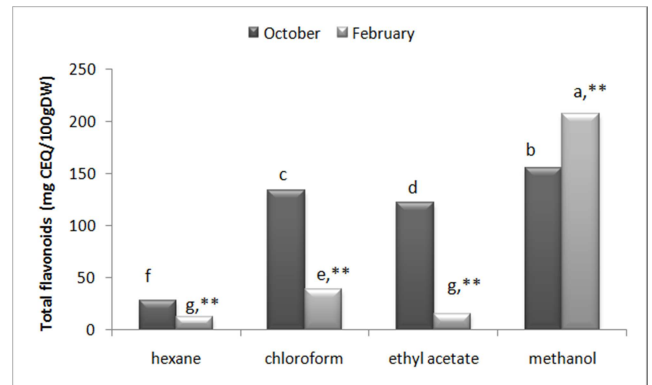
Fig. 4. Total flavonoids content (as catechin equivalents) in extracts from olive leaves sampled in October and February. Values are expressed as means \pm standard deviation ( n = 3 ). Means with different letters were significantly different at the level of p < 0.05 .
