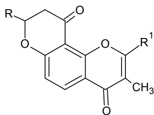
Figure 2. Structural skeleton Chromone derivatives.
