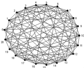
Figure 4. \Gamma(\mathbb{Z}_{21}) .
