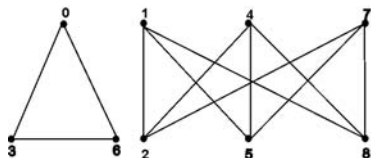
Figure 5. \Gamma(\mathbb{Z}_9) .
