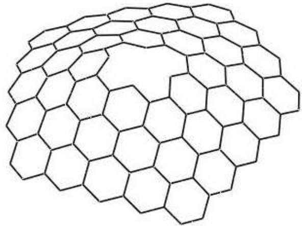
Figure 2. The graph of defect carbon nanocone, CNC_k[n] with k = 13 and n = 3 .
