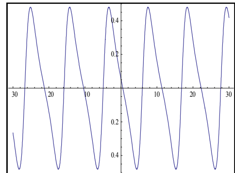
Figure 5. The 3D and 2D surfaces of imaginary part of the analytical solution Eq.(26) by considering the values c = -5, a_2 = 2, -30 < x < 30, -1 < t < 1 , for 3D graphics and t = -0.1 for 2D surfaces.
