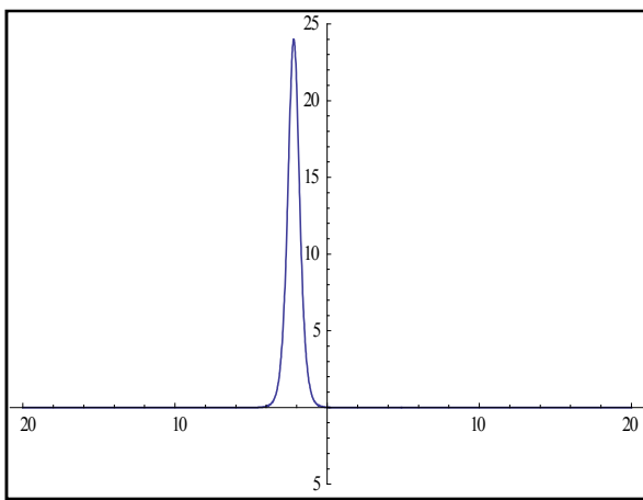
Figure 1. The 3D and 2D surfaces of the analytical solution Eq.(20) being exponential function solution by considering the values b=2, d=-3, c=5, -20 < x < 5, -3 < t < 0 , for 3D graphics and b=2, d=-3, c=5, t=-0.5, -20 < x < 20 for 2D surfaces.
