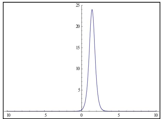
Figure 2. The 3D and 2D surfaces of the analytical solution Eq.(22) being another exponential function solution by considering the values b=d=2, c=-5, -10 < x < 10, -1 < t < 1 , for 3D graphics and b=d=2, c=-5, t=-0.2, -10 < x < 10 for 2D surfaces.
