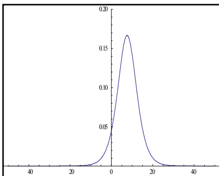
Figure 14. The 3D and 2D surfaces of the analytical solution Eq.(38) being a new exponential function solution by considering the values c = d = -1 , a_3 = -6 , -50 < x < 50 , -20 < t < 20 , for 3D graphics and t = -1
