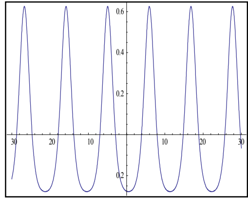
Figure 4. The 3D and 2D surfaces of real part of the analytical solution Eq.(26) by considering the values c = -5, a_2 = 2, -30 < x < 30, -1 < t < 1 for 3D graphics and t = -0.1 for 2D surfaces.
