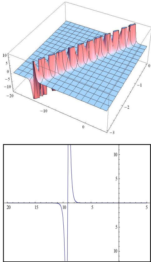
Figure 11. The 3D and 2D surfaces of real part of the analytical solution Eq.(32) by considering the values b=2, c=5, a_4=3, -20 < x < 5, -3 < t < 0 for 3D graphics and t=-2 for 2D surfaces.
