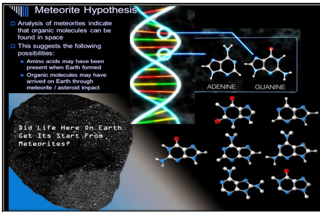
Figure 2. Meteorite containing Guanine and Adenine (Courtesy: NASA).
