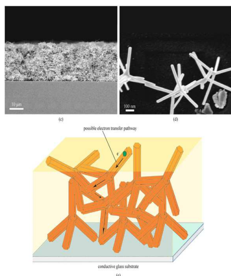
Figure 9. ZnO nanotetrapods structures [13]
