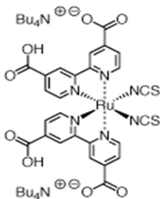
Figure 4. Chemical structure of N719 dye.
