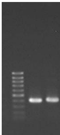
Fig. 2. The result of electrophoresis of the PCR products, on the agarose gel %1.
