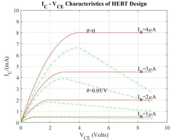
Figure 13. Voltage-Current Characteristics.
