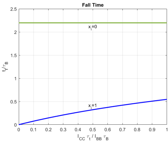
Figure 12. Fall Time. [16].
