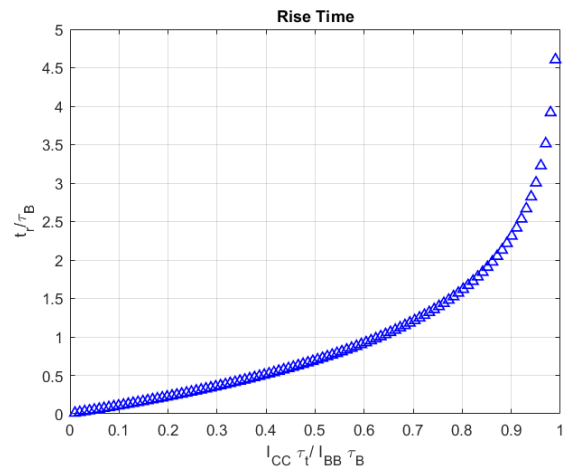
Figure 10. Rise Time. [16].
