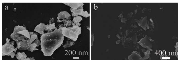
Figure 1. The SEM of (a) fresh sample; (b) the sample after catalytic reaction.
