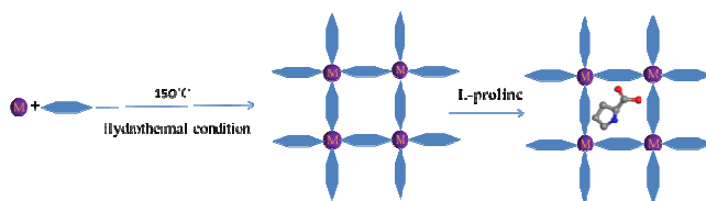
Scheme 1. Synthesis and detection of Ca-L-tart.
