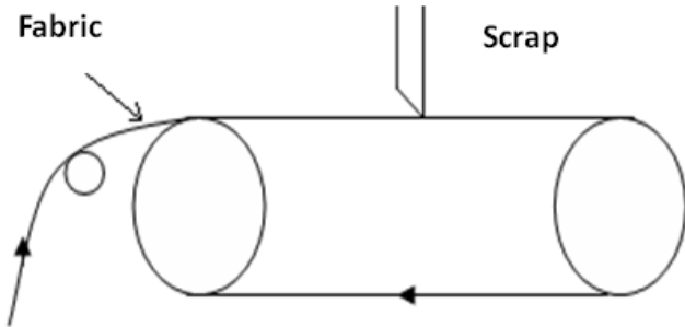
Fig. 1. Fabric coating using a regulated pressure device
