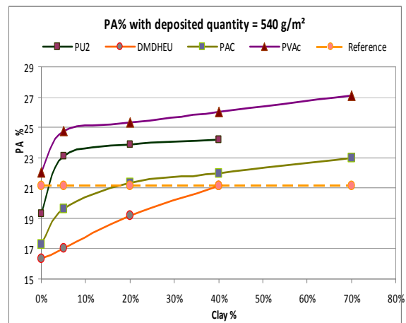
Fig. 3. AP % of coated fabric through resin/clay in terms of the clay rate.
