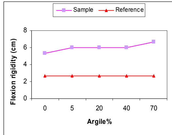
Fig. 7. Rigidity of the coated fabric with PVAc /clay in terms of clay rate.
