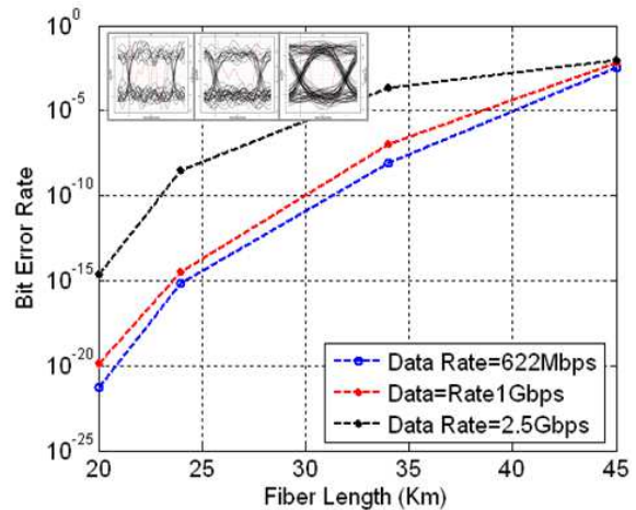
Figure 10. BER versus fiber length at 0 dBm and different Bit rates (Hybrid TDM/DWDM-based PRT is considered).
