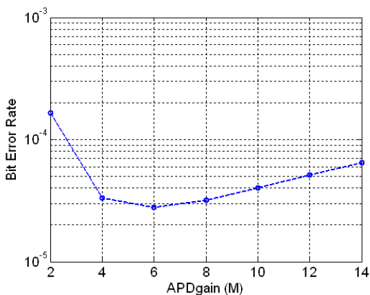
Figure 11. BER versus APD gain (M) at 10 Gbps, 24 kmd, and 2 dBm (Hybrid TDM/DWDM-based PRT is considered).
