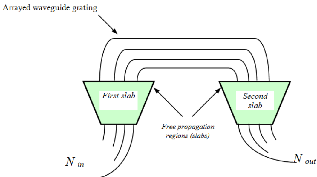
Figure 1. N \times N AWG architecture.
