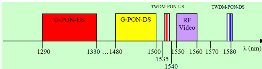
Figure 7. (c). The third option (C-minus/L-minus wavelength plan).
