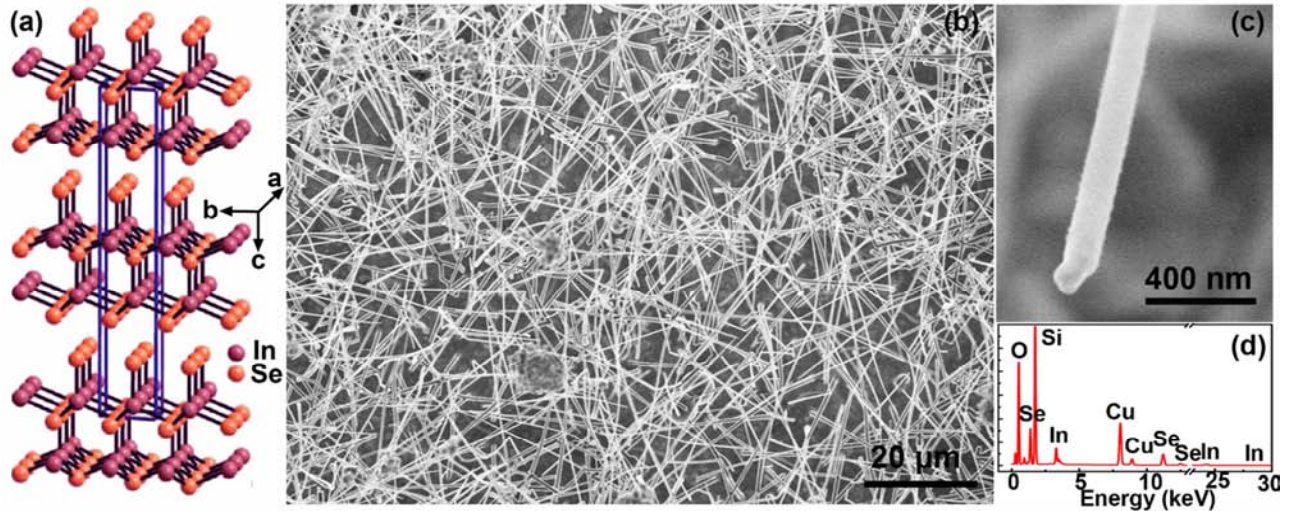
Figure 1. (a) Atomic model of \text{In}_2\text{Se}_3 layered structure. (b, c) SEM of as-grown nanowires. (d) EDS collected from single nanowire dispersed on a copper foil.
