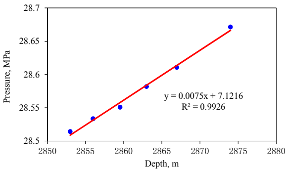
Fig. 10. MDT Test Regression Curve of L 1 , II.
