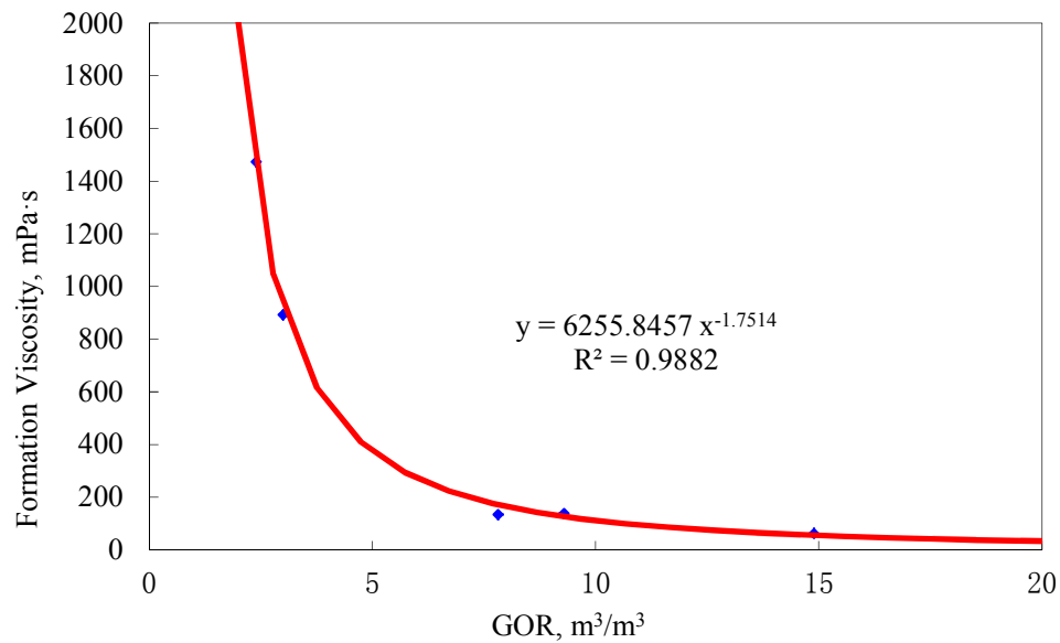
(b) Heavy Oil Reservoir(GOR is less than 15m 3 /m 3 )
