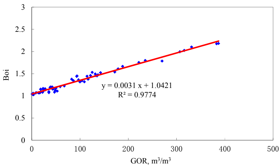
Fig. 6. Boi and GOR Relationship Chart in Beibuwan Basin.
