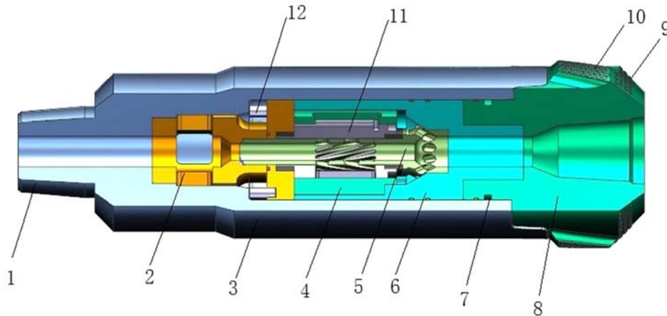
Figure 1. Structure diagram of self-exciting torkbuster.
