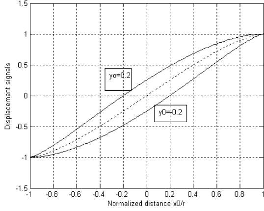
Fig.3. The normalized displacement signals \varepsilon_x (dotted) and \varepsilon_\zeta for two values of y_0/r , as a function of the normalized distance x_0/r .
