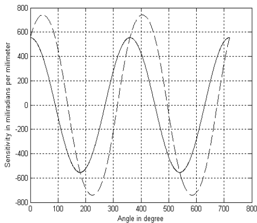
Fig.7. The sensitivity for (1+1,--), and (2+2) configurations as a function of angle \varphi_0 , for \rho_0/r=0.2 , and r=2.25\text{mm} .
