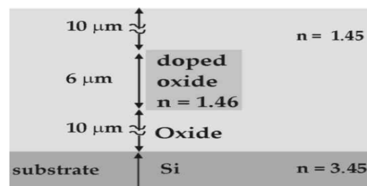
Figure 1. Cross-section of a waveguide fabricated in silica on silicon.
