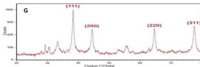
Fig 3. F and G, XRD pattern of respectively E and D sample after heating
