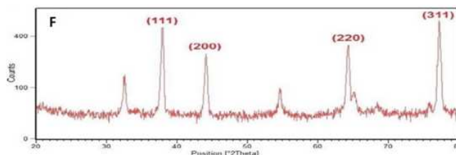
Fig 2. XRD pattern of sample that synthesis in dark environment
