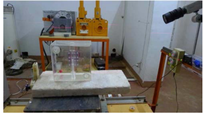
Figure 2. Irradiation of TLDs at SSDL (INSTN-Madagascar).
