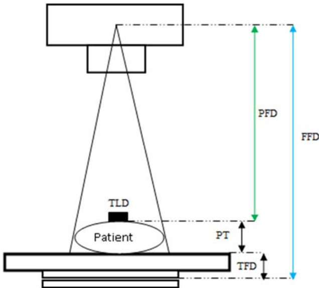
Figure 1. Patient ESAC measurement using TLD.
