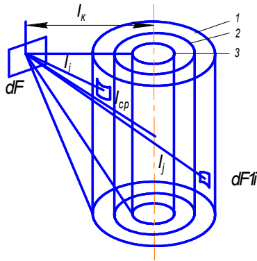
Fig. 4. To the calculation of radiant fluxes from coaxial cylinder 1 – 3, l_i , l_p , l_{am} – the distance from surface elements and arithmetic mean distance to dF calculated area.
