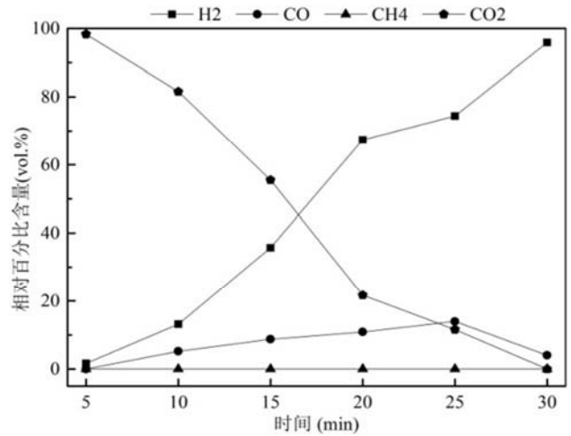
(c) 焙烧温度800°C
