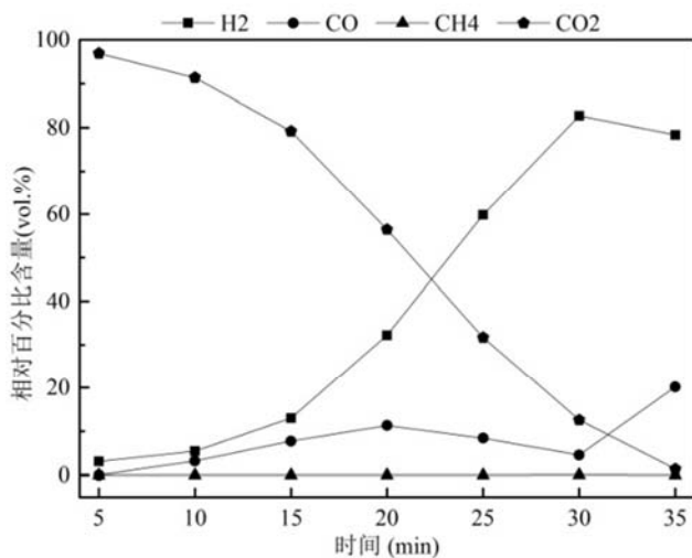
(a) 负载量80wt%
