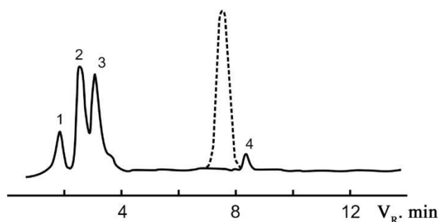
Fig 4. Chromatographic curves of the products of biodegradation of hydroquinone 3-keto- cis, cis -muonic acid (1), 4-hydroxy- cis, cis -muonic acid (2), polyaldehyde 4-hydroxy- cis, cis -muonic acid (3), hydroxyhydroquinone (4), (dotted lines – hydroquinone).
