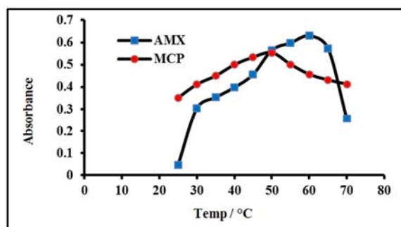
Figure 6. Effect of equilibration temperature on the absorbance and extractability of azo dye product [Conditions: For AMX: 1.0 µg mL -1 , diazotized MCP; 9x10 -5 M, Na 2 CO 3 ; 3.0x10 -3 M, TX-114; 1.0%, 20 min incubation time. For MCP; 0.88 µg mL -1 , AMX; 9.53x10 -6 M, Na 2 CO 3 ; 1.0x10 -3 M, TX-114; 0.6%, 20 min incubation time].
