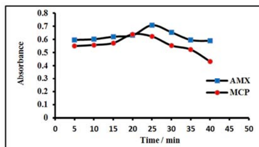
Figure 7. Effect of incubation time on absorbance and extractability of azo dye product [Conditions: For AMX: 1.0 µg mL -1 , diazotized MCP; 9x10 -5 M, Na 2 CO 3 ; 3.0x10 -3 M, TX-114; 1.0%, CPT; 60°C. For MCP; 0.88 µg mL -1 , AMX; 9.53x10 -6 M, Na 2 CO 3 ; 1.0x10 -3 M, TX-114;0.6 % CPT; 50 °C].
