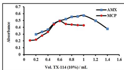
Figure 5. Effect of the TX-114 amount on absorbance and extractability of azo dye product [Conditions: For AMX: 1.0 µg mL -1 , diazotized MCP; 9x10 -5
