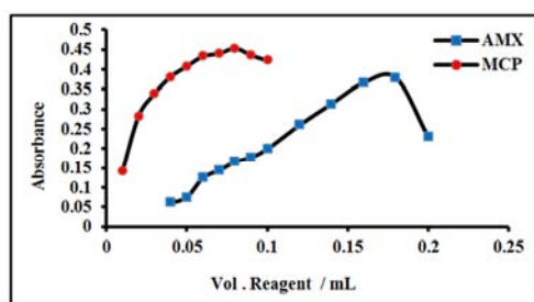
Figure 4. Effect of the reagents concentration on absorbance and extractability of azo dye product [Conditions: For AMX: 1.0 µg mL -1 , Na 2 CO 3 ; 3.0x10 -3 M, TX-114; 0.5% CPT; 65°C and 20 min incubation time. For MCP; 0.88 µg mL -1 .Na 2 CO 3 ; 1.0x10 -3 M, TX-114; 0.5%, CPT; 65°C and 20 min incubation time].
