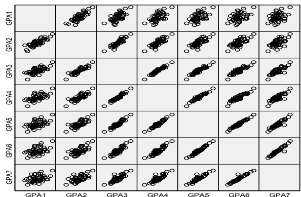
Figure 5. The scatter plot of the correlation structure
