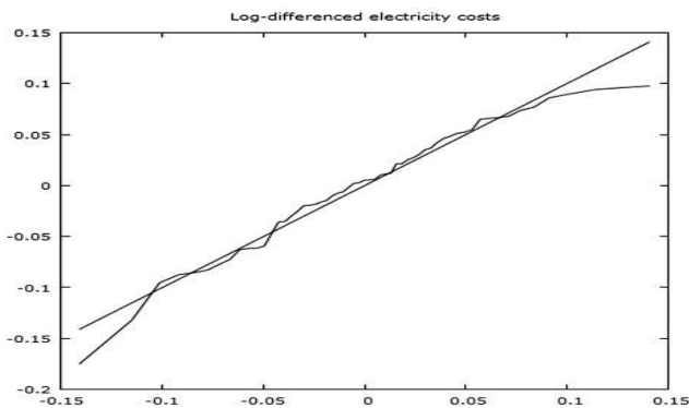
Fig 5. The normal QQ curve for the log-differenced electricity cost
