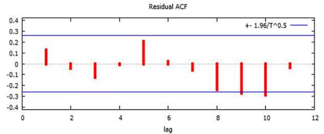
Figure 4. ACF of Log-Differenced costs
