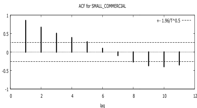
Figure 3. ACF for electricity cost
