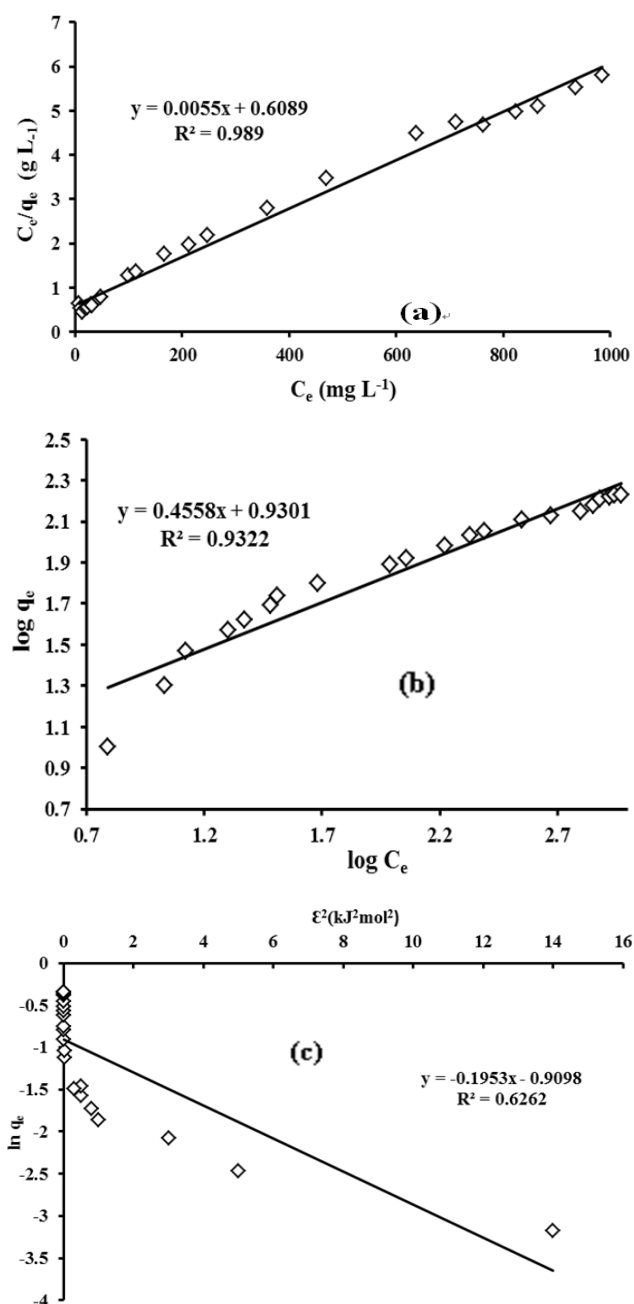
Figure 4. Isotherms models: (a) Langmuir; (b) Freundlich and (c) D-R for U(VI) sorption onto Lewatit MonoPlus M500.
