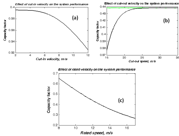
Figs.3. Effect of wind turbine speeds on capacity factor.
